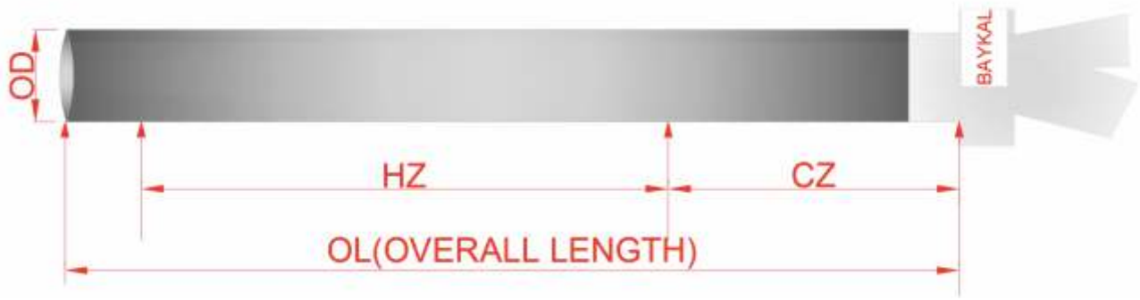
Dimensional drawing of SIC electric rod
